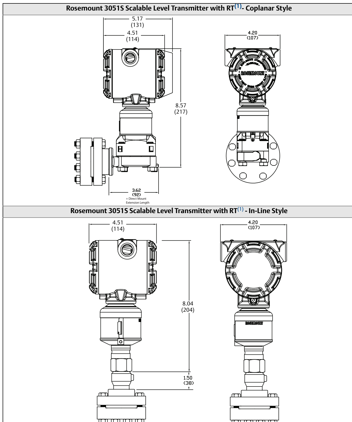
Figure 17. Rosemount 3051S Scalable Level Transmitter with RT Seal
