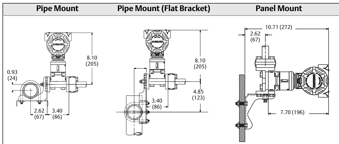
Figure 7. Traditional Mounting Configurations
