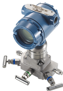
3051S Coplanar Pressure Transmitter
