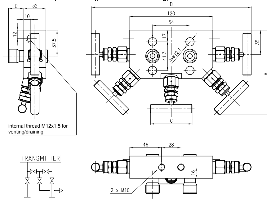
Figure 10 - Five-way valve set (964 25.. AS2), dimensional drawing, scheme
