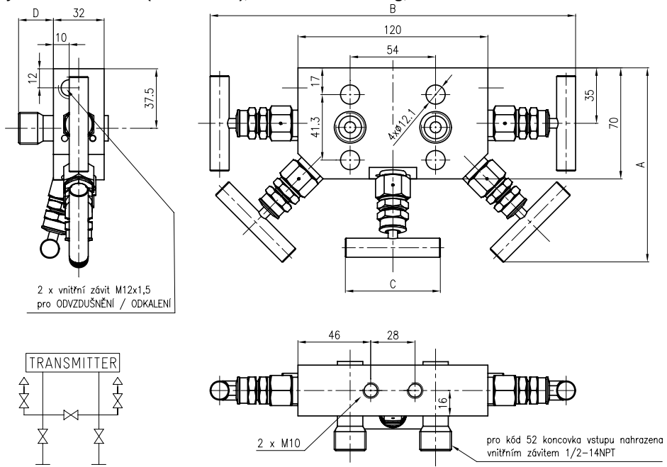
Figure 9 - Five-way valve set (964 25.. AS1), dimensional drawing, scheme
