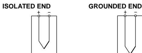
FIGURE 1 – DESIGN OF MEASURING END OF JACKET THERMOCOUPLES (SCHEME DIAGRAM)
