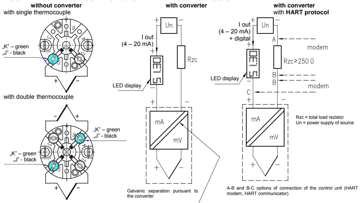
FIGURE 1 - SCHEME OF CONNECTION OF TEMPERATURE SENSORS
