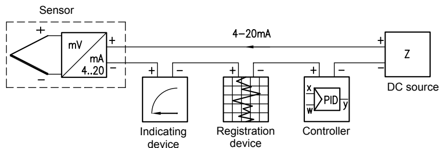
FIGURE 2 - EXAMPLE OF OPERATION CONNECTION OF TEMPERATURE SENSOR WITH CONVERTER IN LOOP 4 - 20 mA
