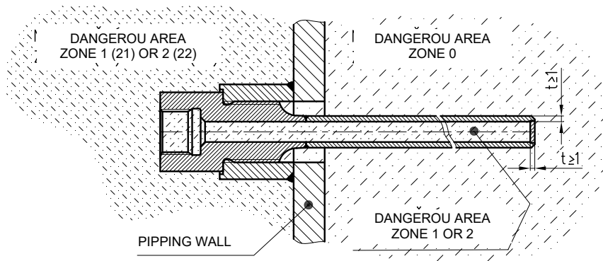
FIGURE 8 – MARK OF NON-EXPLOSIVENESS
