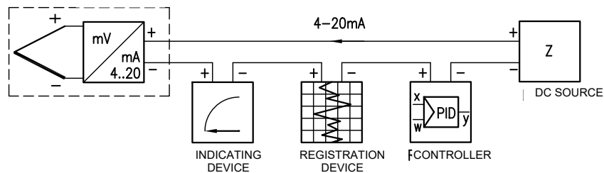
FIGURE 5 - EXAMPLE OF OPERATION CONNECTION OF TEMPERATURE SENSOR WITH CONVERTER IN LOOP 4 - 20 mA SENSOR
