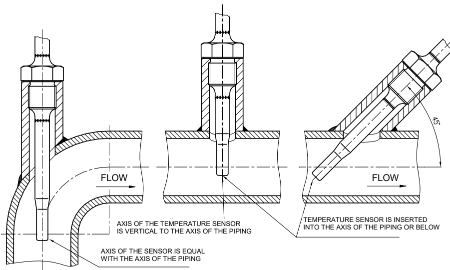
FIGURE 3 – EXAMPLES OF INSTALLATION OF DIRECT AND OBLIQUE NIPPLES PURSUANT TO EN1434-2
