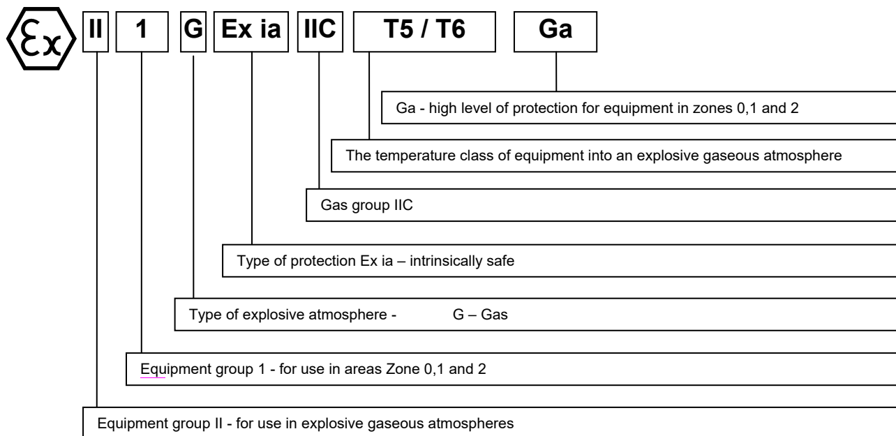
FIGURE 9 - INTRINSICALLY SAFE MARKING
