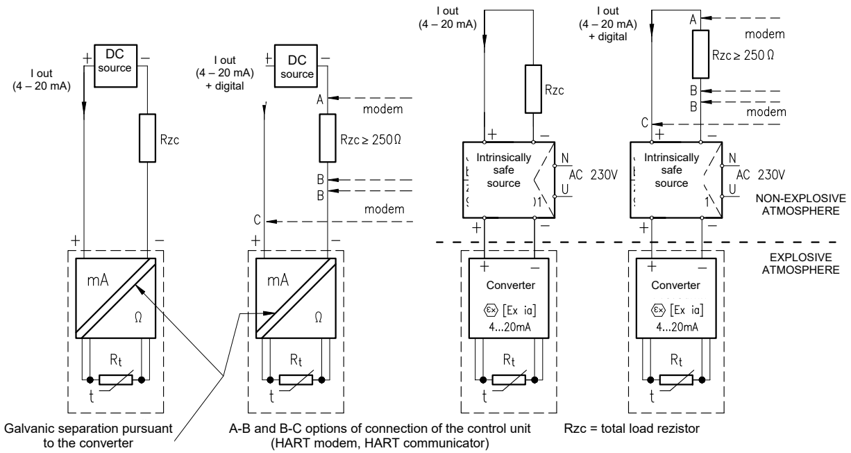
FIGURE 5 - EXAMPLE OF OPERATION CONNECTION OF TEMPERATURE SENSOR WITH CONVERTER IN LOOP 4 - 20 mA SENSOR
