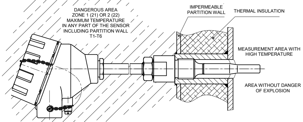
FIGURE 6 – EXAMPLE OF INSTALLATION OF TEMPERATURE SENSORS Ex d TO THERMOWELL ČSN (in case a higher limit of the measurement range is required on a level exceeding the required temperature class)
