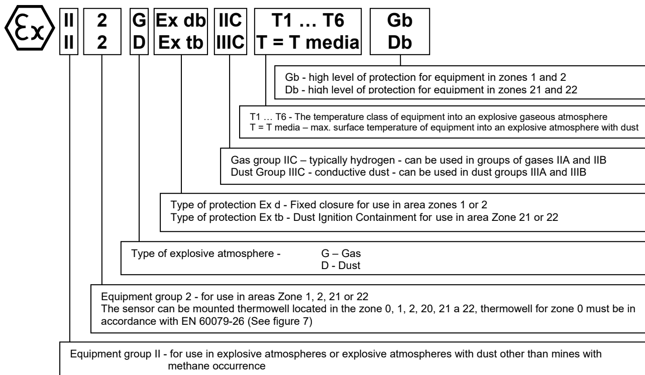
FIGURE 8 – MARK OF NON-EXPLOSIVENESS
