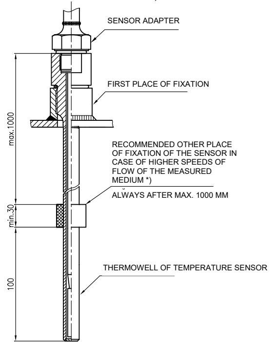
FIGURE 2 - PROPOSAL OF SECURING THERMOWELL OF TEMPERATURE SENSORS Ex d (for nominal lengths exceeding 630 mm) Prescribed thermowells of type 991 (pursuant to ON 02 7210, ON 02 7212, ON 02 7215 or ON 02 7217) shall be used.
