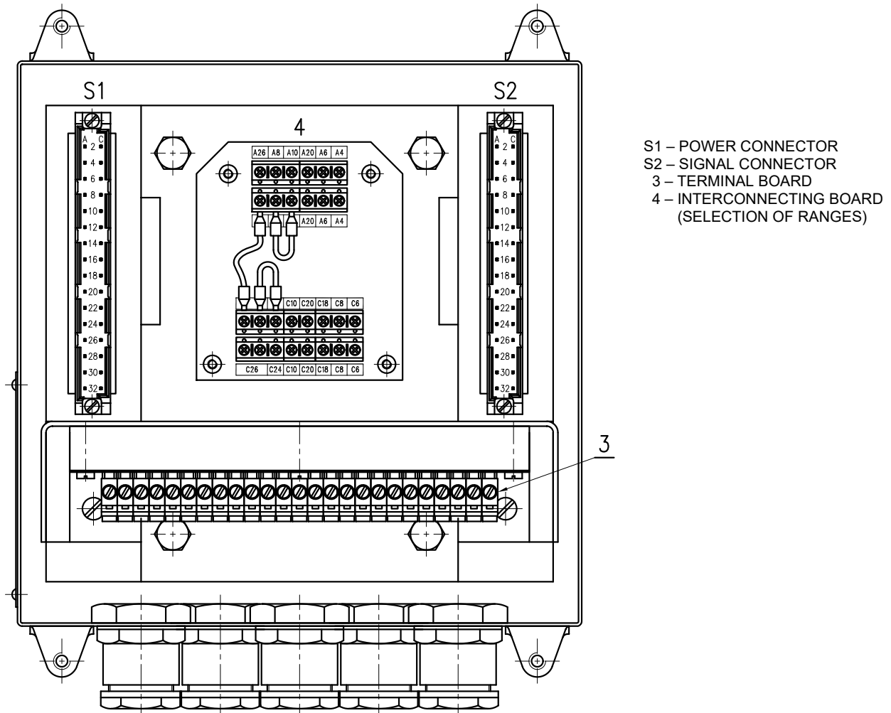
FIGURE 3 - DRAWING OF LOCATION OF CONNECTORS, TERMINAL BOARD AND INTERCONNECTING BAR IN A BOX OF THE CONTROLLERS OF TYPE 511 22 AND 511 25
