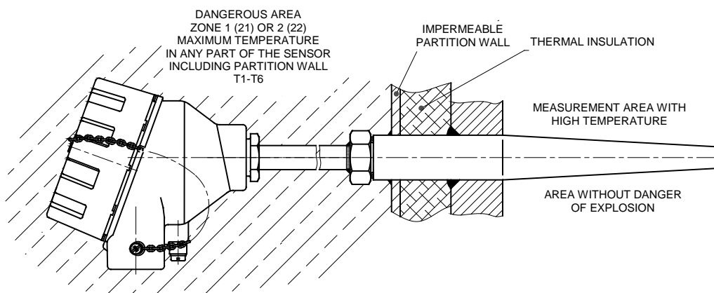
FIGURE 3 – EXAMPLE OF INSTALLATION OF TEMPERATURE SENSORS Ex d TO THERMOWELL DIN
