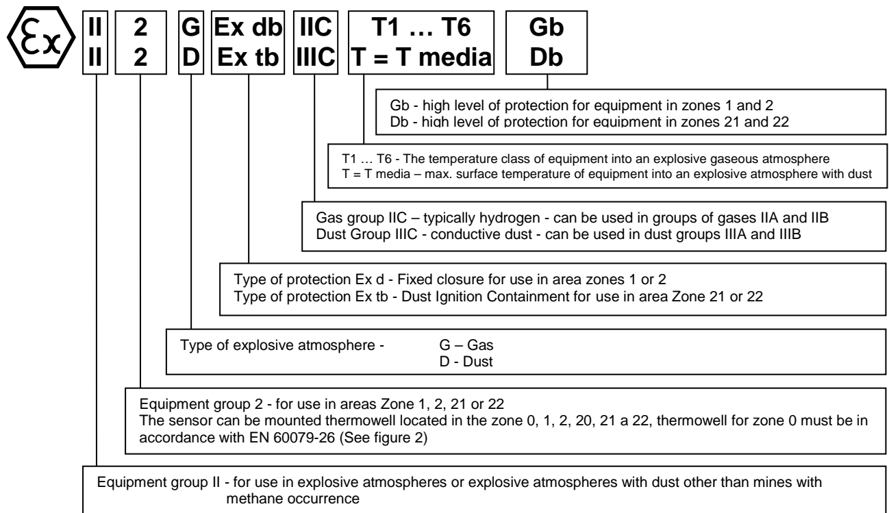
FIGURE 1 – MARK OF NON-EXPLOSIVENESS
