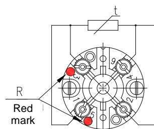
SCHEME OF CONNECTION WITH CONVERTER AND DISPLAY
