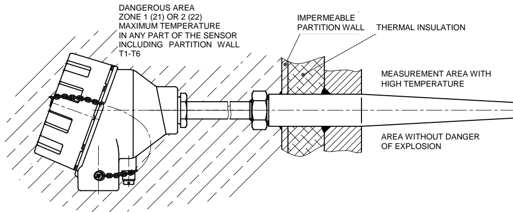
FIGURE 3 – EXAMPLE OF INSTALLATION OF TEMPERATURE SENSORS Ex d TO THERMOWELL DIN (in case a higher limit of the measurement range is required on a level exceeding the required temperature class)
