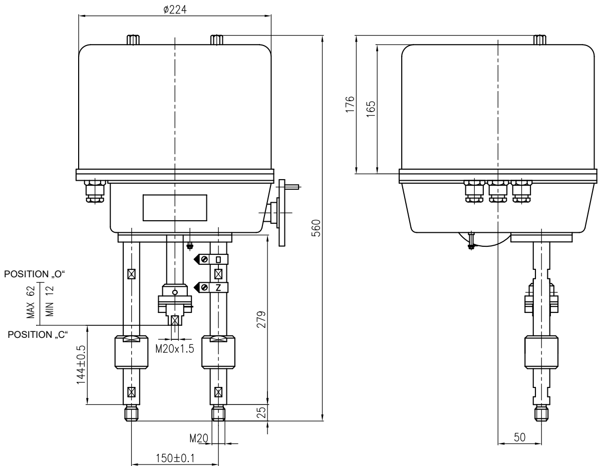
FIGURE 2 - DIMENSIONAL DRAWING - CONNECTION P4
