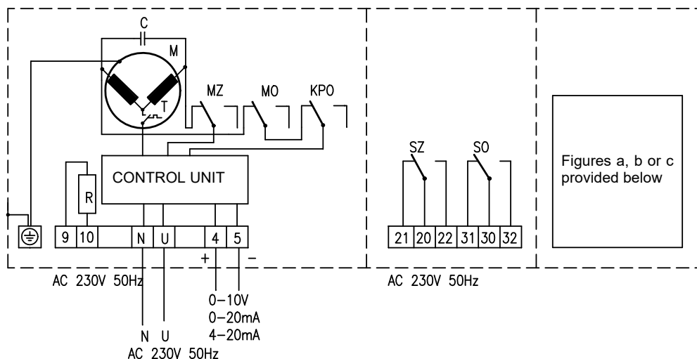
FIGURE 5 - CONNECTION SCHEME AND DRAWING OF TERMINAL BOARD – CONTROL 0-10 V, 0-20 mA, 4-20 mA
