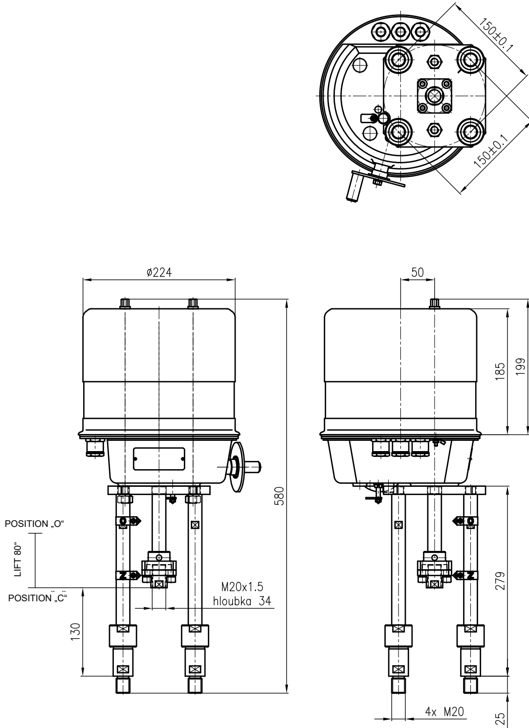
FIGURE 3 - DIMENSIONAL DRAWING - CONNECTION P5 - PITCH 150, 4 COLUMNS M 20, FITTING M20x1,5, LIFT 80
