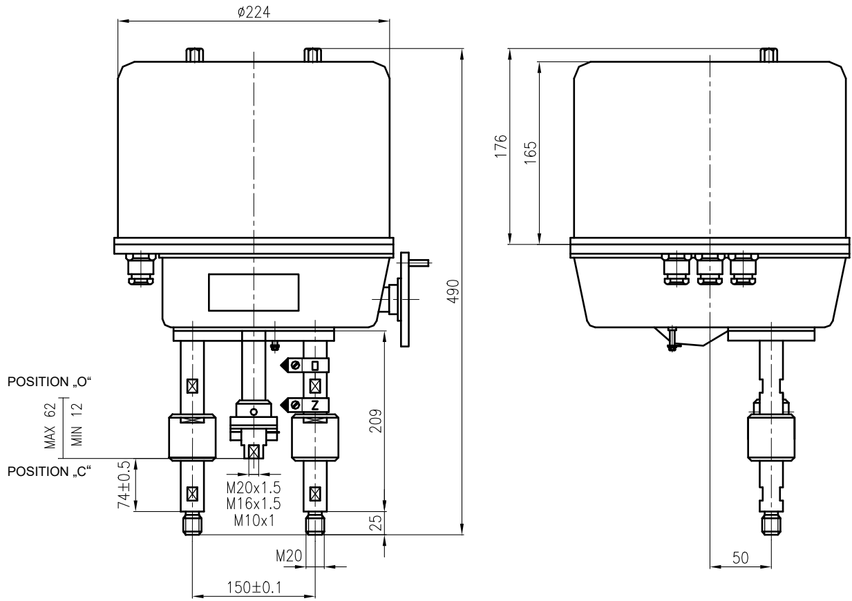
FIGURE 1 - DIMENSIONAL DRAWING - CONNECTION P2 - COUPLING M20X1.5, - CONNECTION P3 - COUPLING M16X1.5 or M10x1
