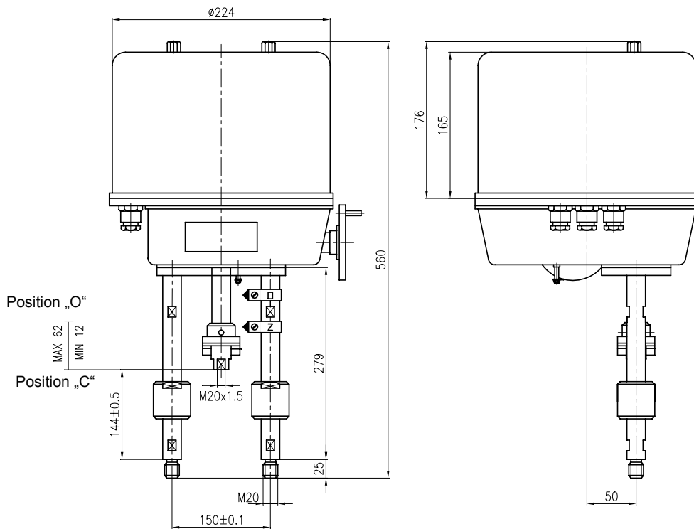
Figure 2 Dimensional drawing - connection P4
