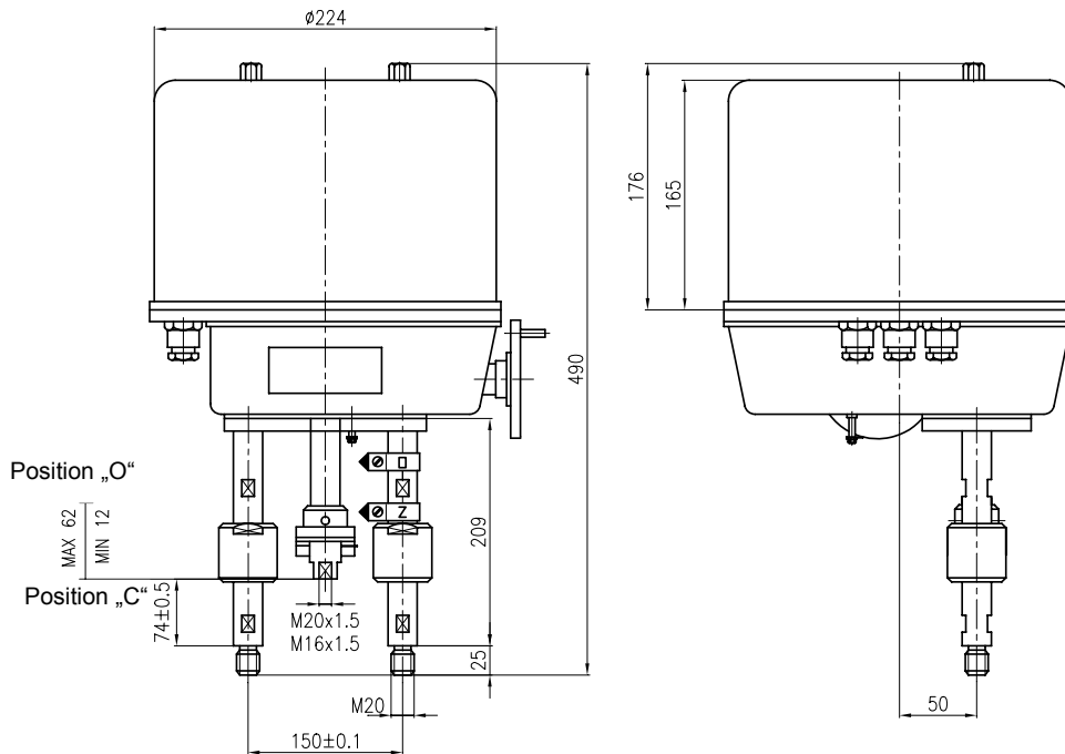
Figure 1 Dimensional drawing - connection P2 - coupling M20x1.5, - connection P3 - coupling M16x1.5
